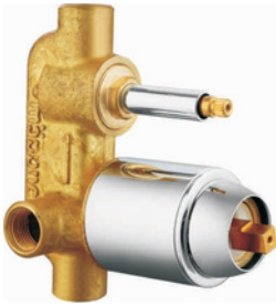
DCB 4534 Concealed Body For High Flow Single Lever Mixer & Diverter (45mm Cartridge) without Exposed Parts ₹ 4500/-
