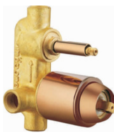
DCB 4032 RG Concealed Body For Single Lever Diverter & Mixer 3 Inlet & 2 Outlet (45mm Cartridge) without Exposed Parts (Rose Gold) ₹ 5500/-
