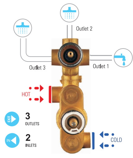
DCB 4023 TH MRP ₹ 11580/- (Chrome)
